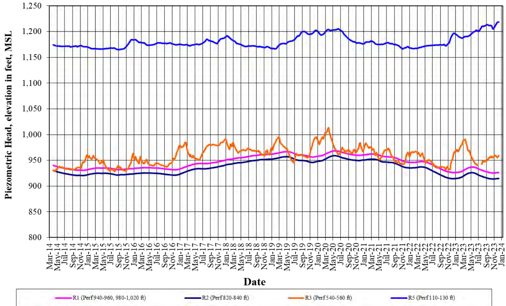
Figure 4 Piezometric Head for Multiple Depth Monitoring Well VDC Recharge Basin Well (8S/1W-6R1-6) April 24, 2014 through December 31, 2023
