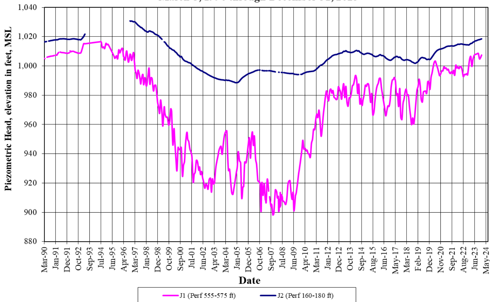
Figure 2 Piezometric Head for Multiple Depth Monitoring Well Wolf Valley Well (8S/2W-20J1-2) March 5, 1990 through December 31, 2023
