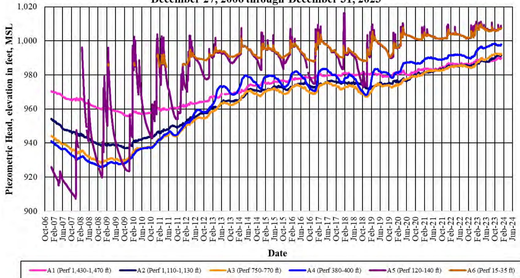
Figure 1 Piezometric Head for Multiple Depth Monitoring Well Pala Park Well (8S/2W-19A1-6) December 27, 2006 through December 31, 2023
