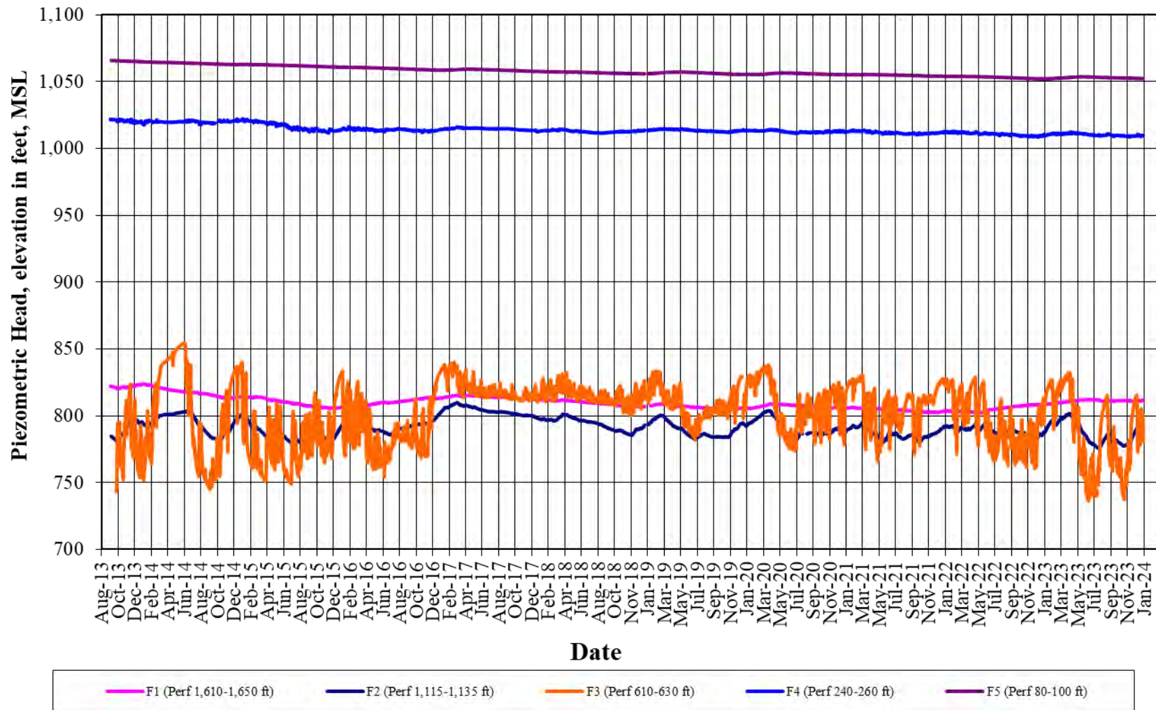
Figure 3 Piezometric Head for Multiple Depth Monitoring Well Temecula Creek Well (8S/2W-15F1-5) September 28, 2013 through December 31, 2023
