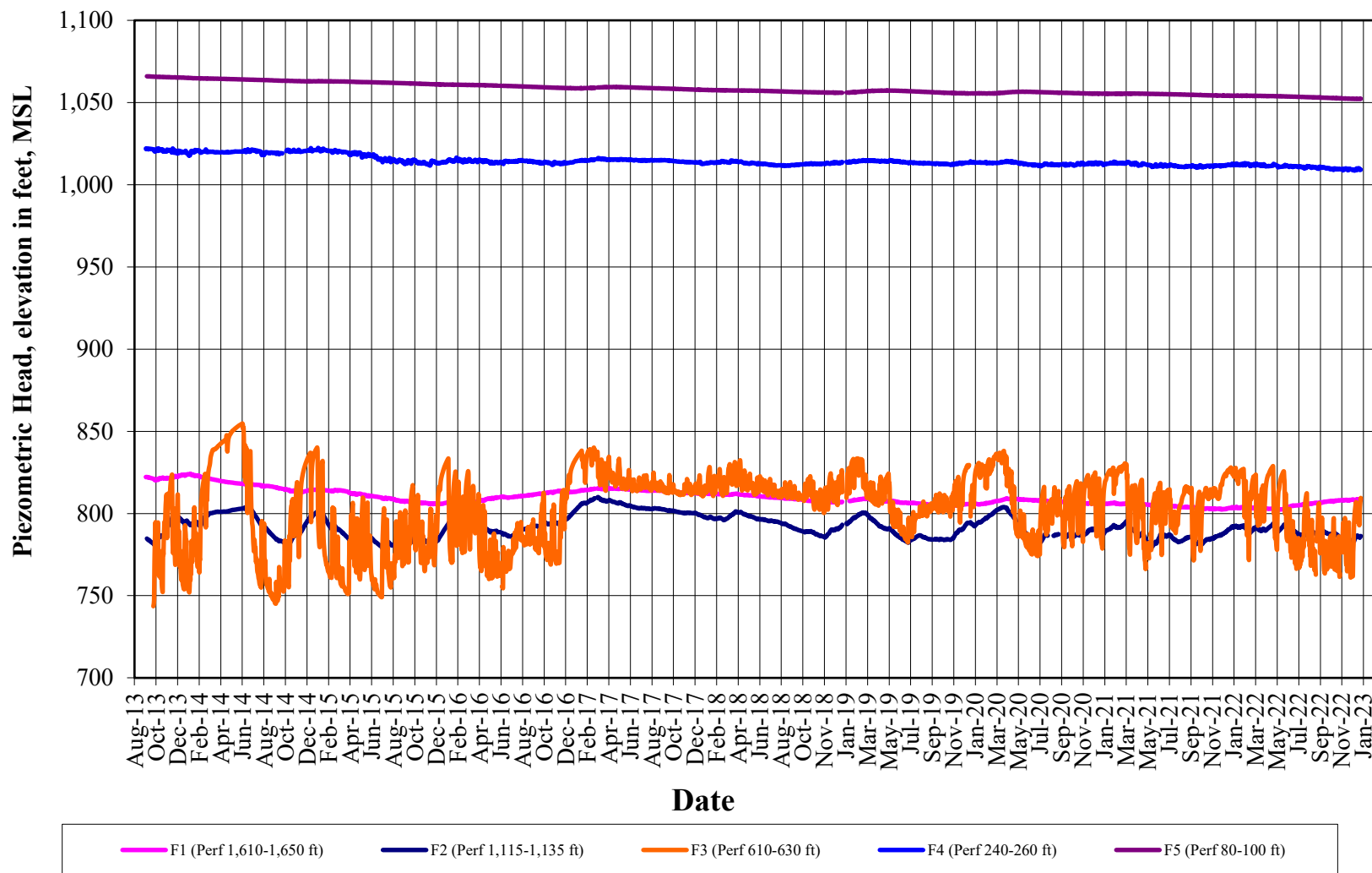
Figure 3 Piezometric Head for Multiple Depth Monitoring Well Temecula Creek Well (8S/2W-15F1-5) September 28, 2013 through December 31, 2022
