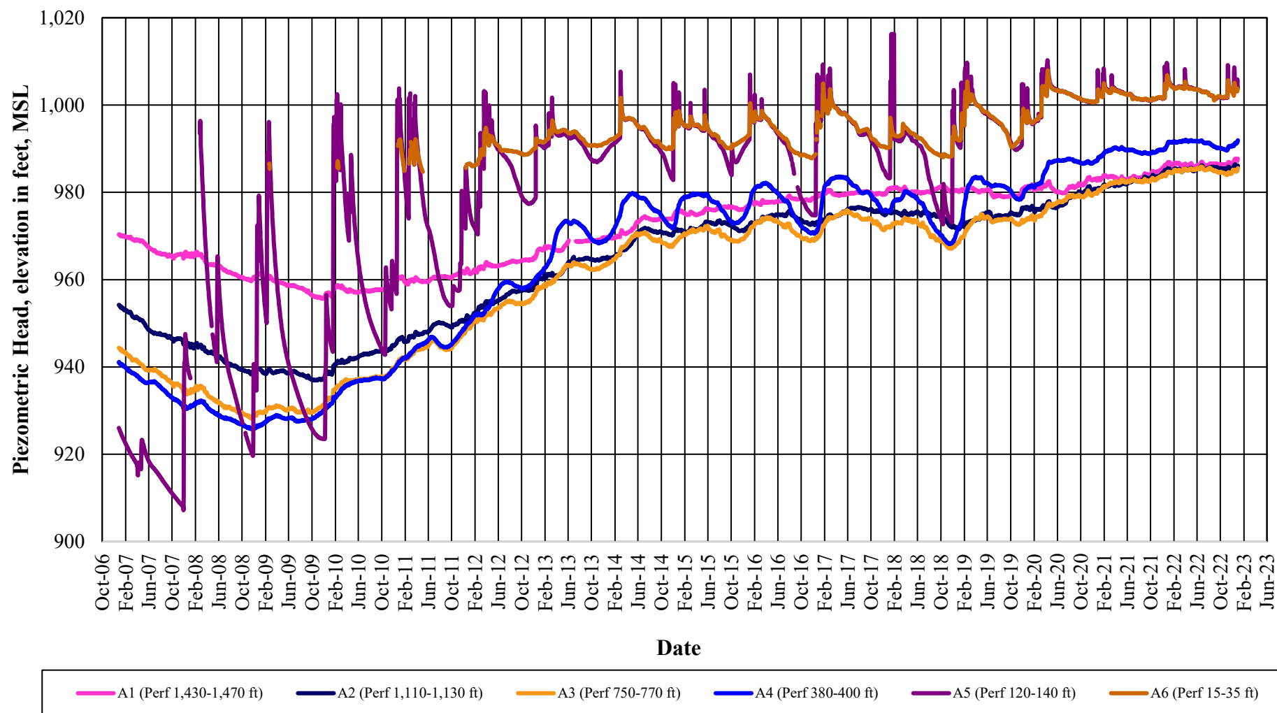
Figure 1 Piezometric Head for Multiple Depth Monitoring Well Pala Park Well (8S/2W-19A1-6) December 27, 2006 through December 31, 2022
