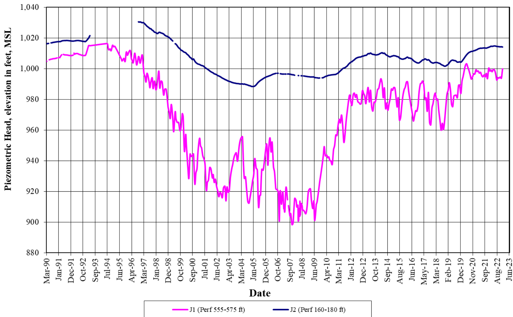
Figure 2 Piezometric Head for Multiple Depth Monitoring Well Wolf Valley Well (8S/2W-20J1-2) March 5, 1990 through December 31, 2022
