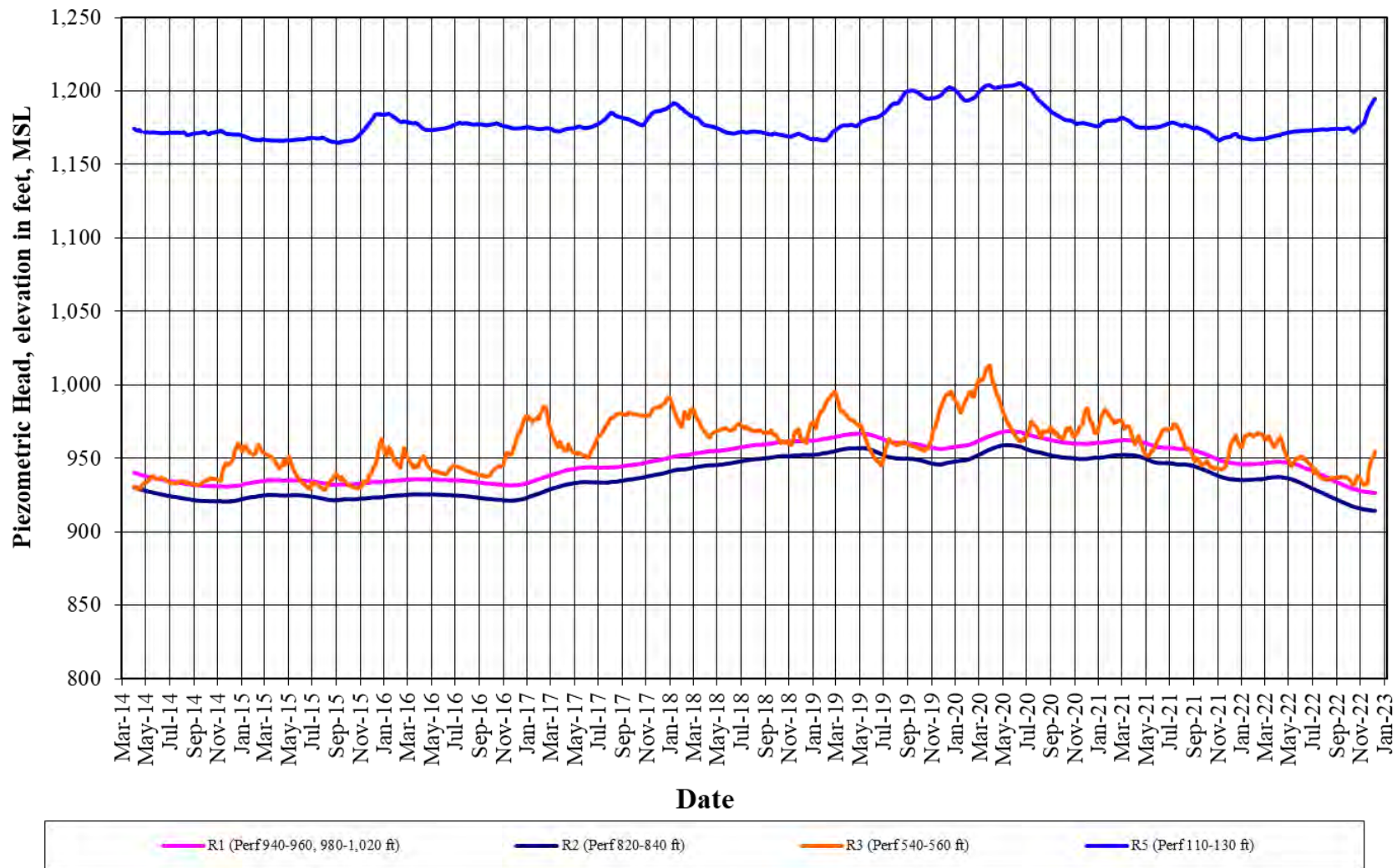
Figure 4 Piezometric Head for Multiple Depth Monitoring Well VDC Recharge Basin Well (8S/1W-6R1-6) April 24, 2014 through December 31, 2022
