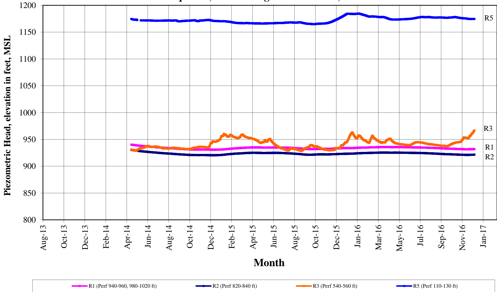
Figure 4 Piezometric Head for Multiple Depth Monitoring Well VDC Recharge Basin Well (8S/1W-6R1-6) April 24, 2014 through December 31, 2016
