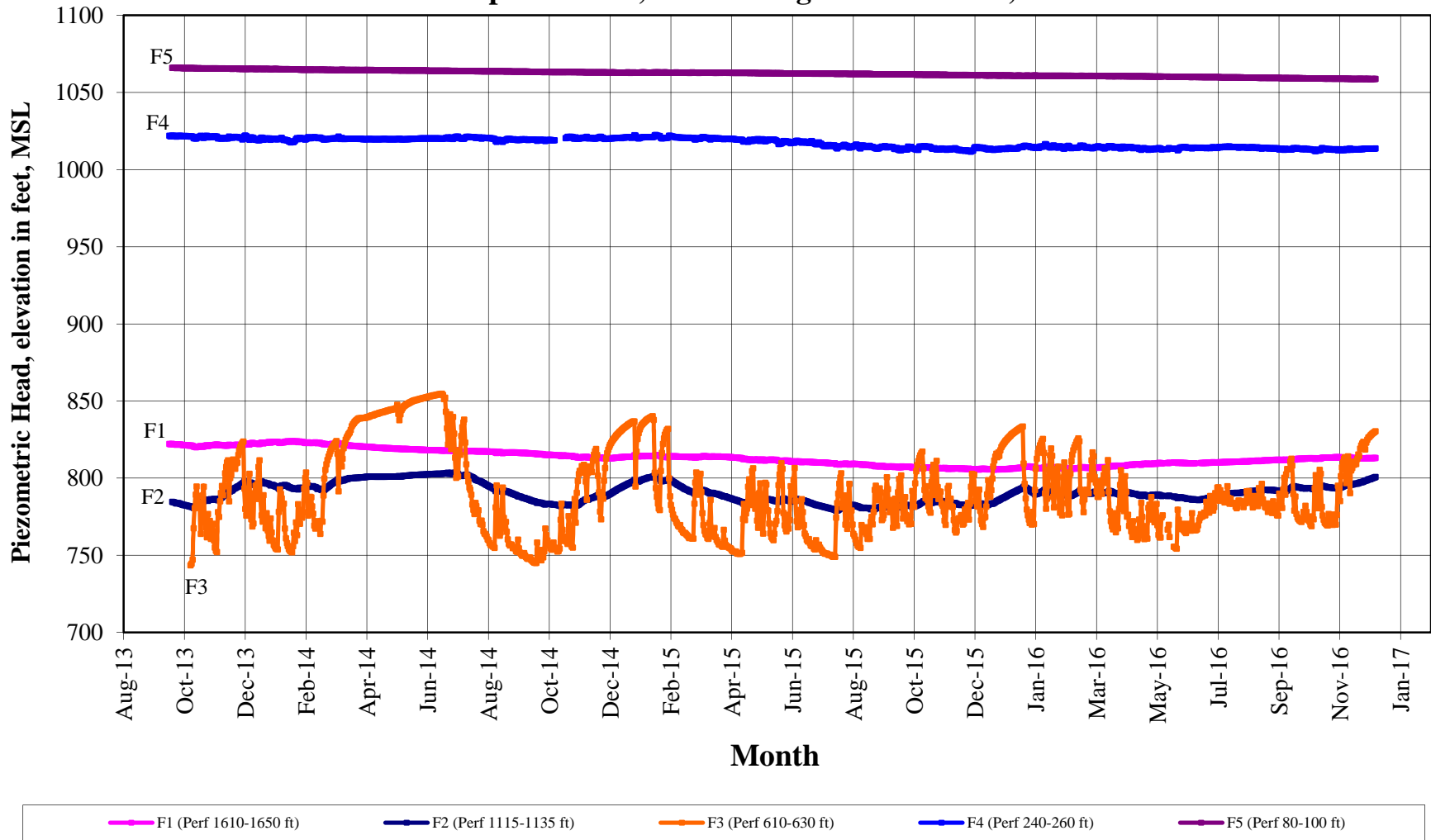
Figure 3 Piezometric Head for Multiple Depth Monitoring Well Temecula Creek Well (8S/2W-15F1-5) September 28, 2013 through December 31, 2016
