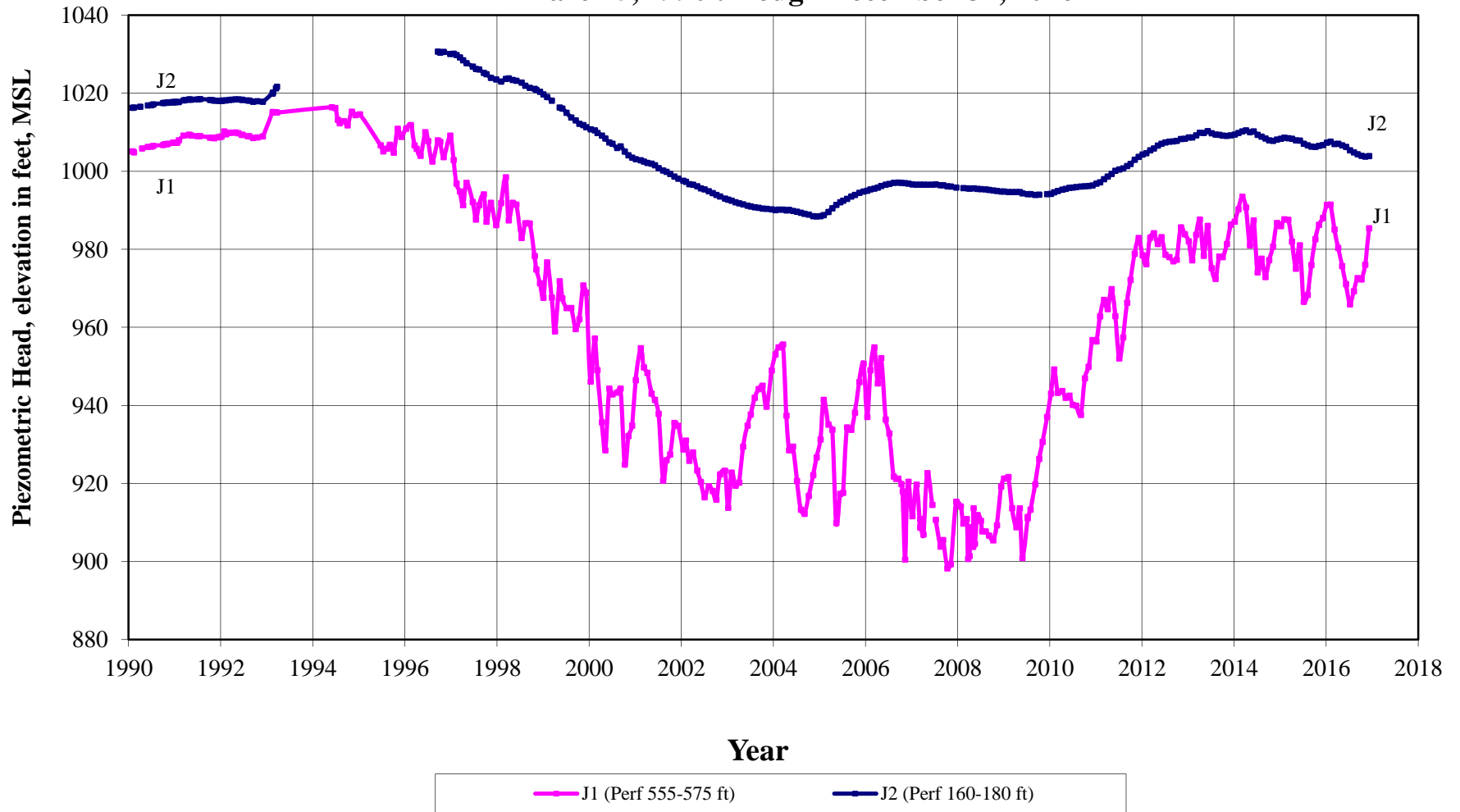
Figure 2 Piezometric Head for Multiple Depth Monitoring Well Wolf Valley Well (8S/2W-20J1-2) March 5, 1990 through December 31, 2016
