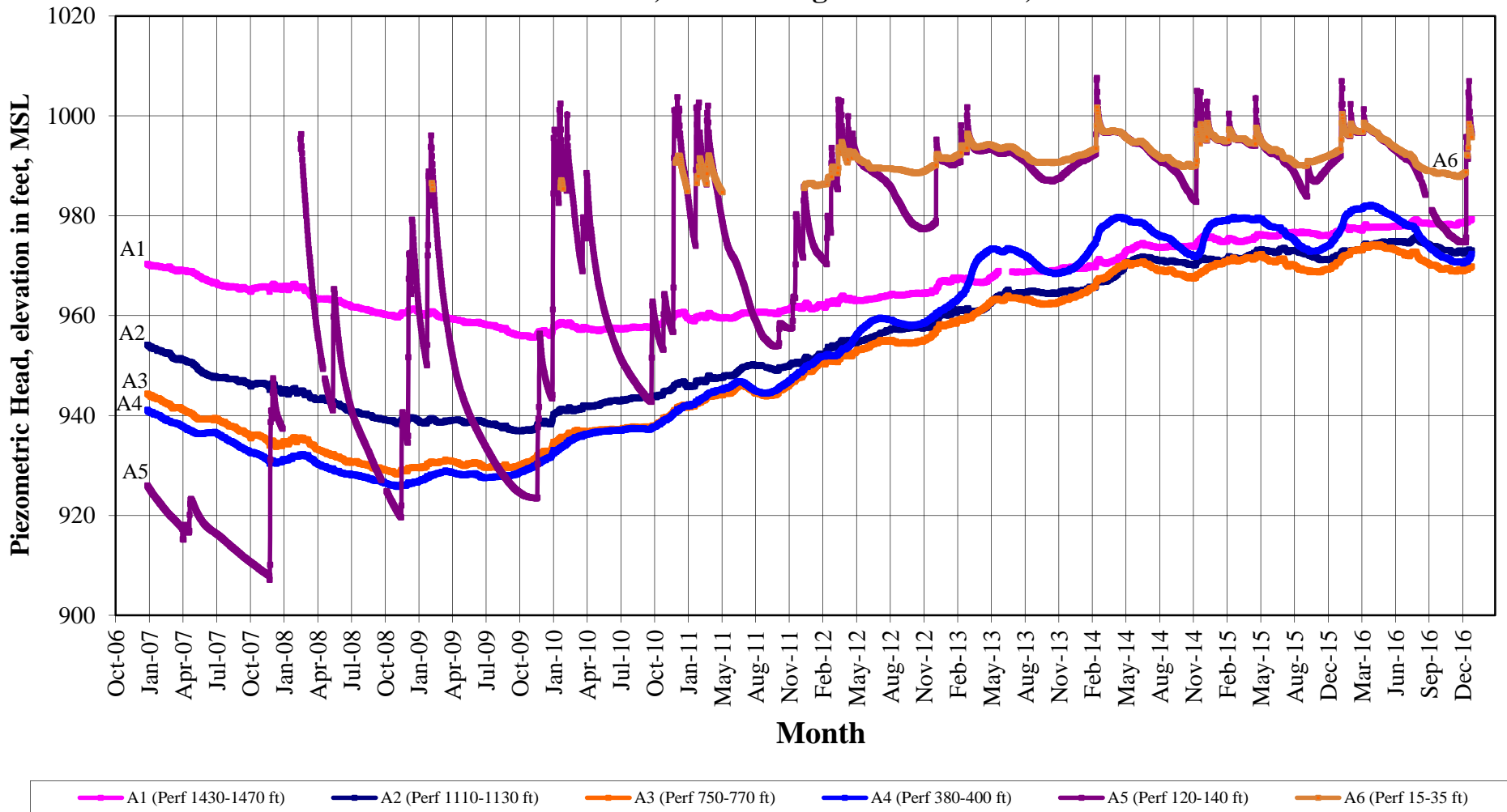
Figure 1 Piezometric Head for Multiple Depth Monitoring Well Pala Park Well (8S/2W-19A1-6) December 27, 2006 through December 31, 2016
